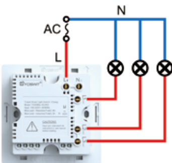
Connection 1: Without neutral wire
