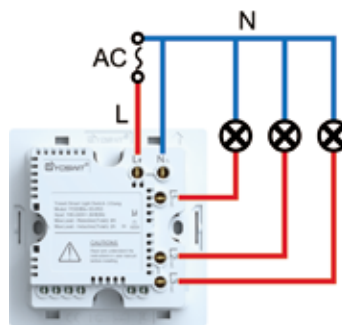
Connection 2: With neutral wire
